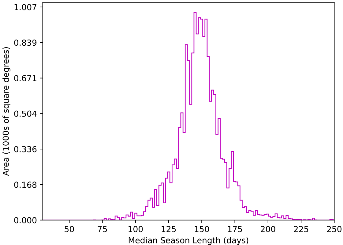
too_100_1v3.4_10yrs WFD z band: Median Season Length
