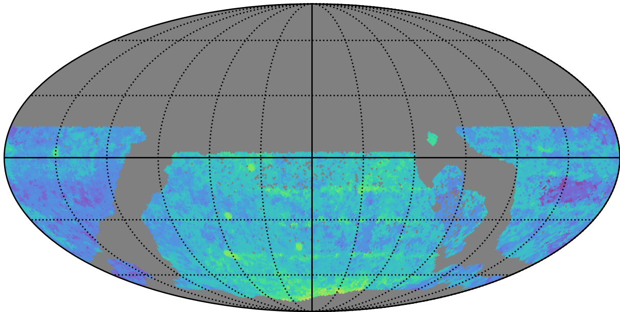
too_100_1v3.4_10yrs WFD y band: Median Season Length
