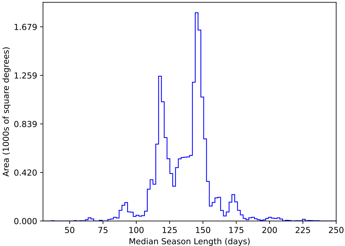
too_100_1v3.4_10yrs WFD y band: Median Season Length
