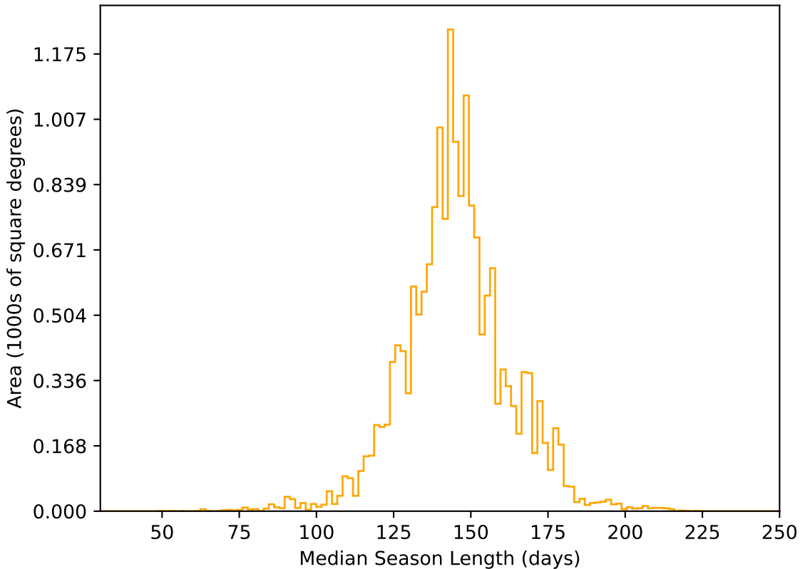
too_100_1v3.4_10yrs WFD r band: Median Season Length
