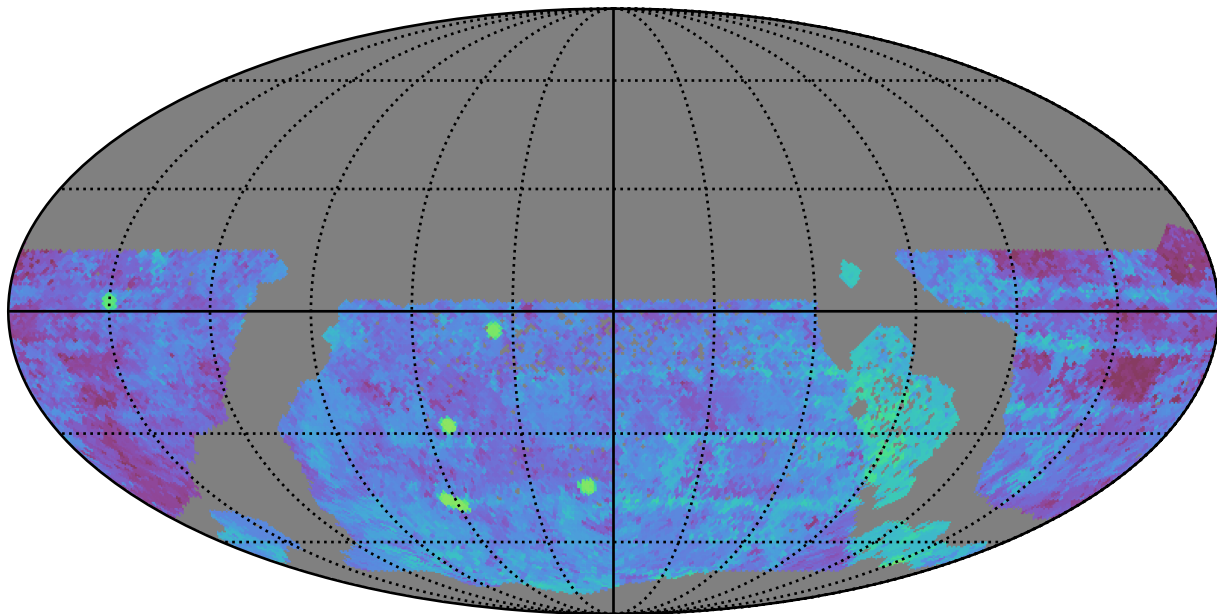
too_100_1v3.4_10yrs WFD g band: Median Season Length
