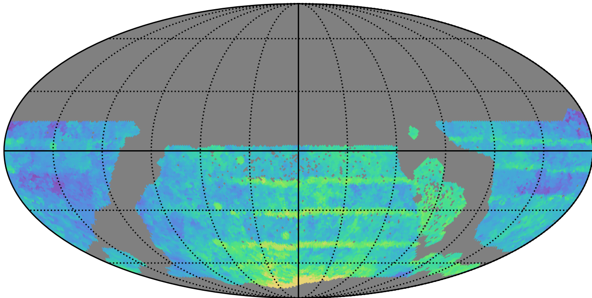
too_100_1v3.4_10yrs WFD all bands: Median Season Length
