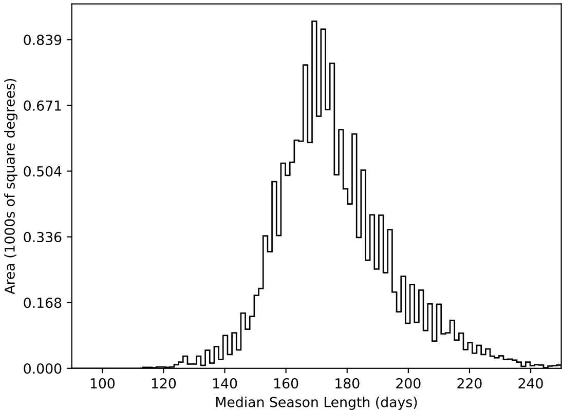
too_100_1v3.4_10yrs WFD all bands: Median Season Length
