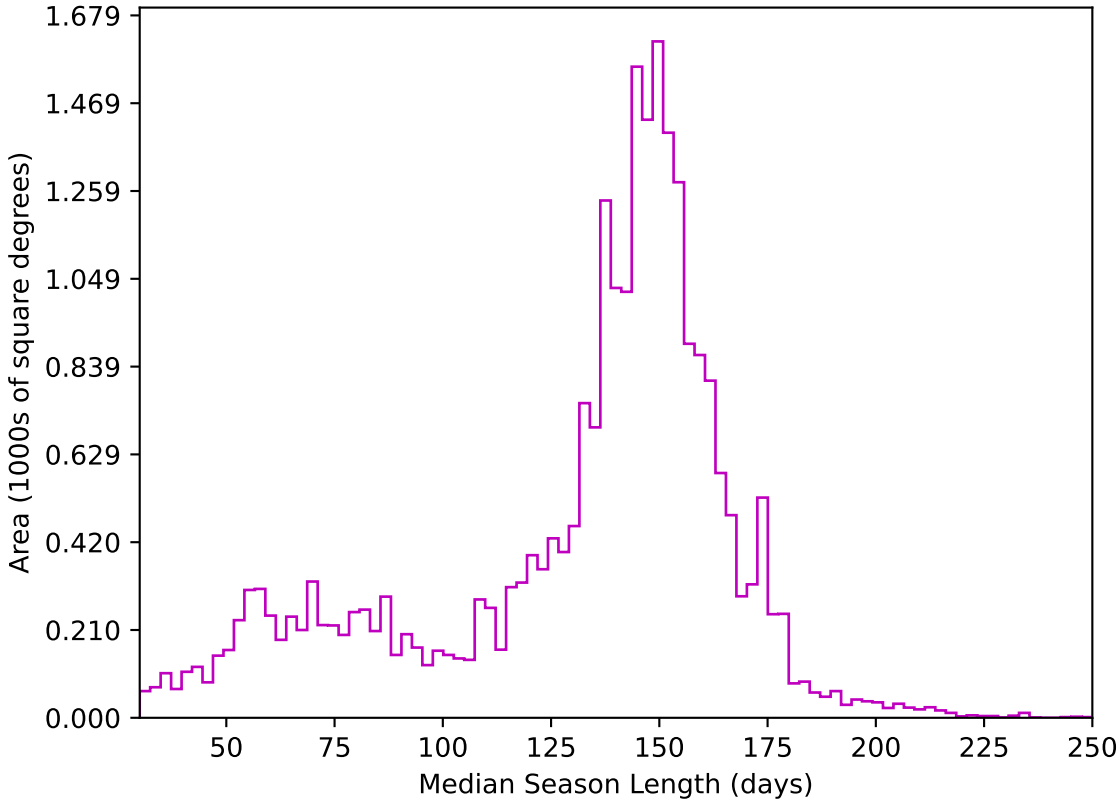
too_100_1v3.4_10yrs All sky z band: Median Season Length
