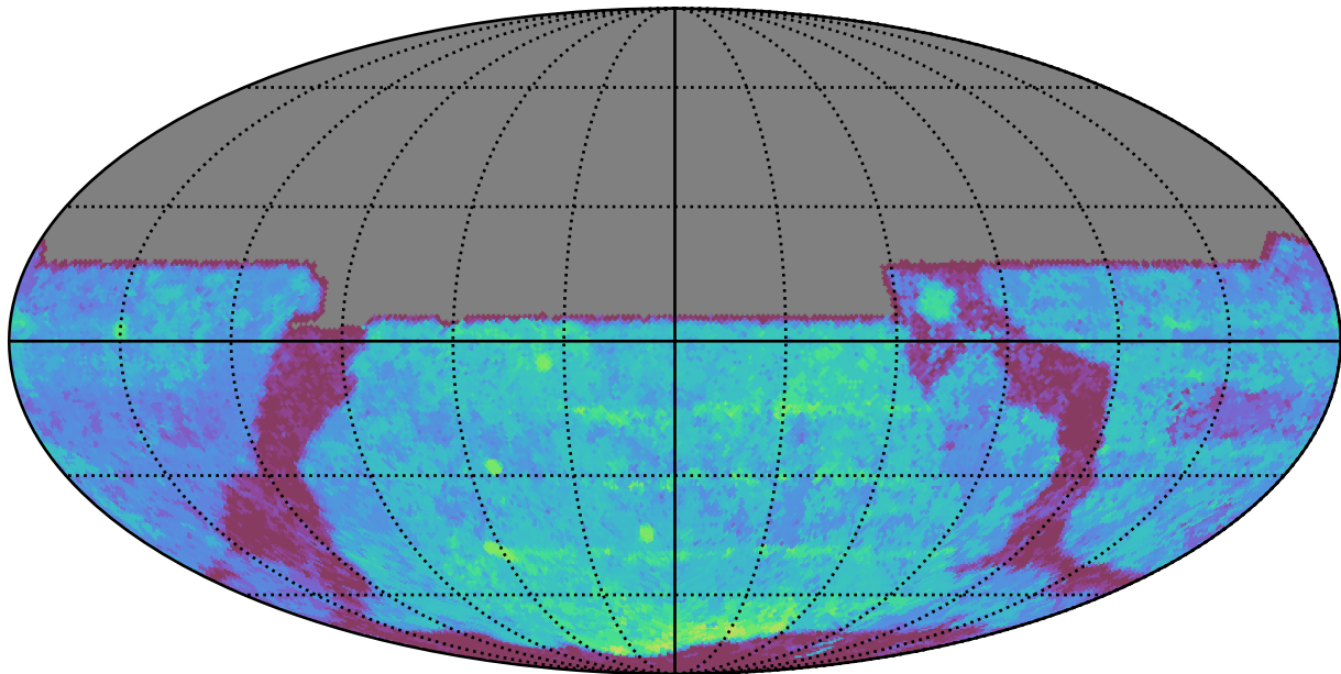
too_100_1v3.4_10yrs All sky y band: Median Season Length
