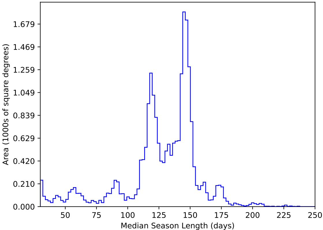
too_100_1v3.4_10yrs All sky y band: Median Season Length
