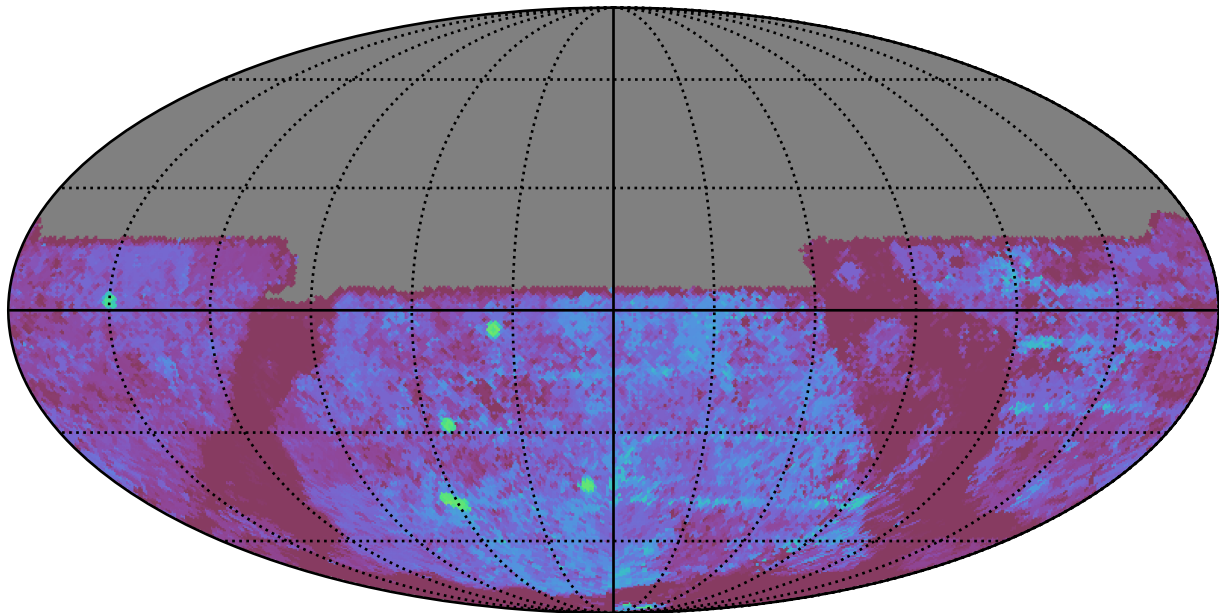
too_100_1v3.4_10yrs All sky u band: Median Season Length
