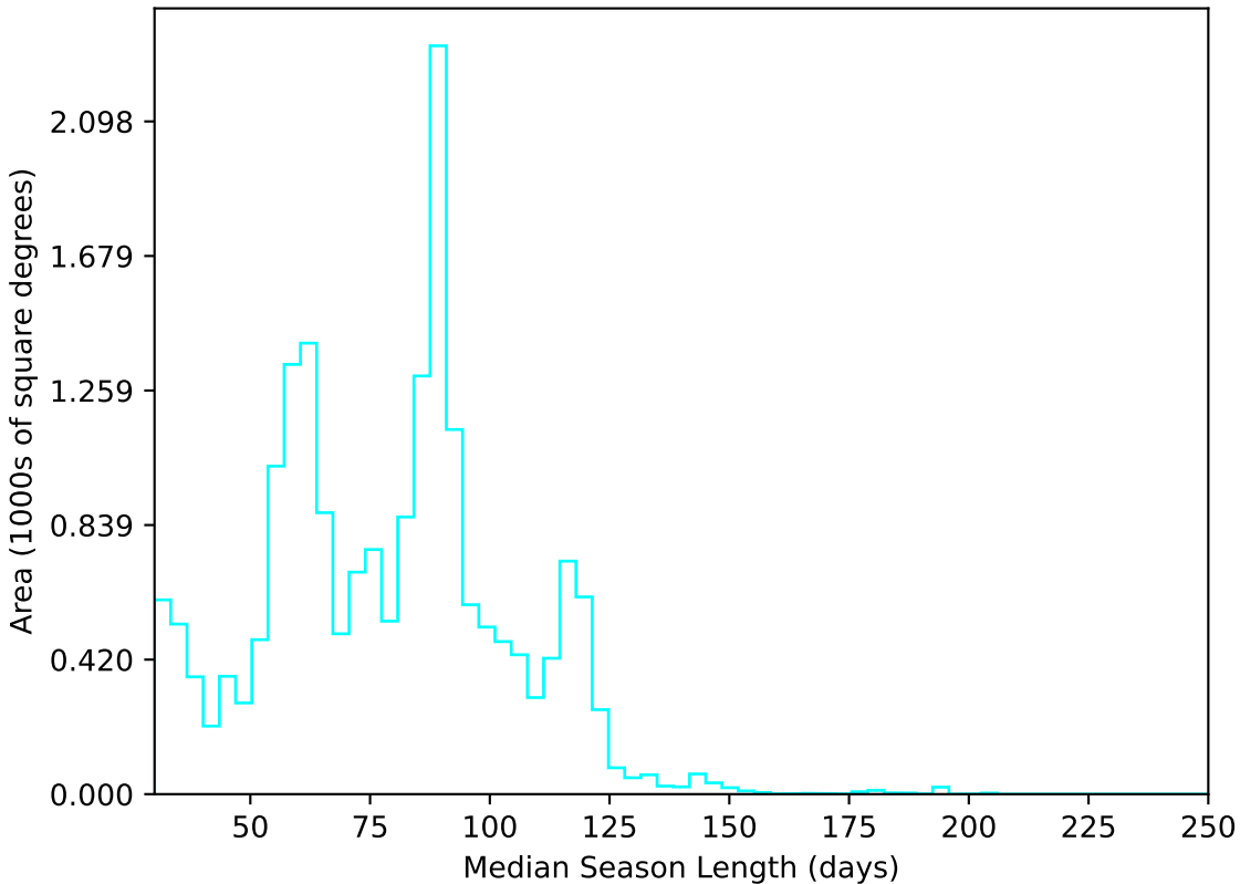
too_100_1v3.4_10yrs All sky u band: Median Season Length
