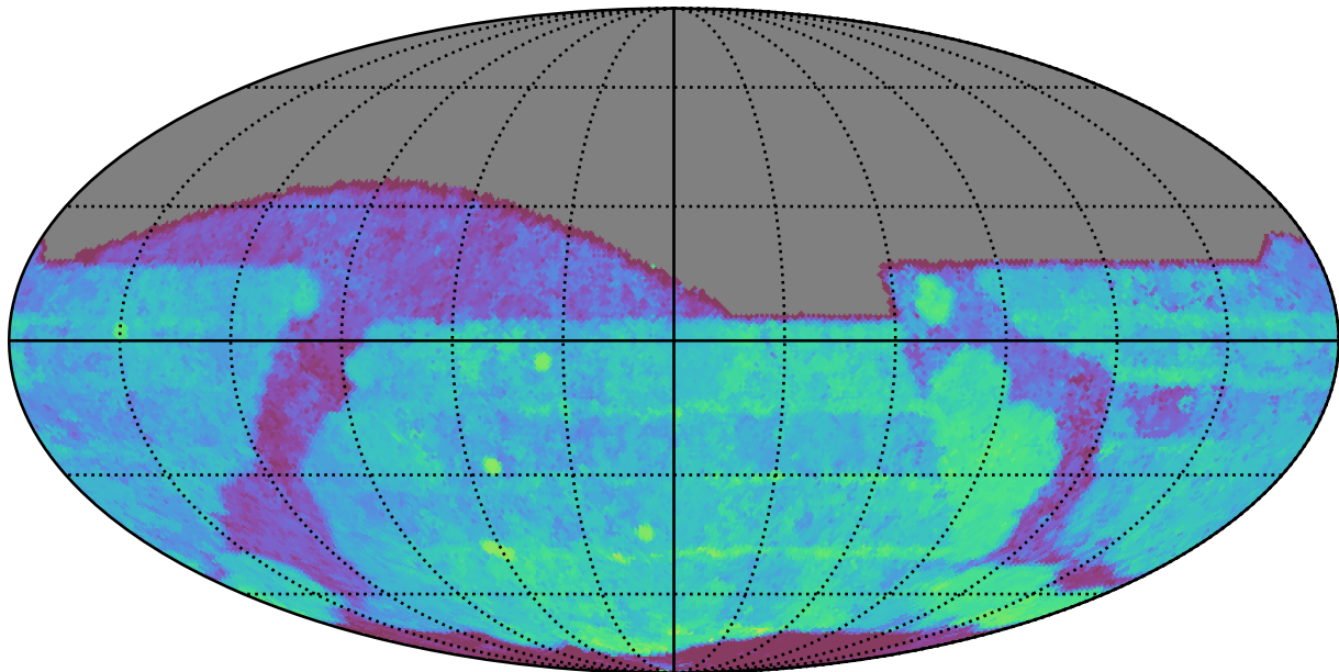
too_100_1v3.4_10yrs All sky r band: Median Season Length
