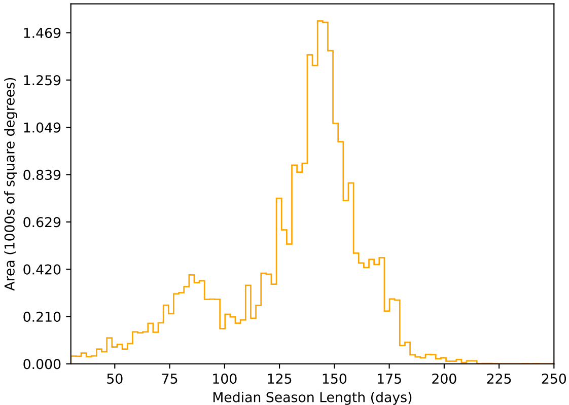
too_100_1v3.4_10yrs All sky r band: Median Season Length
