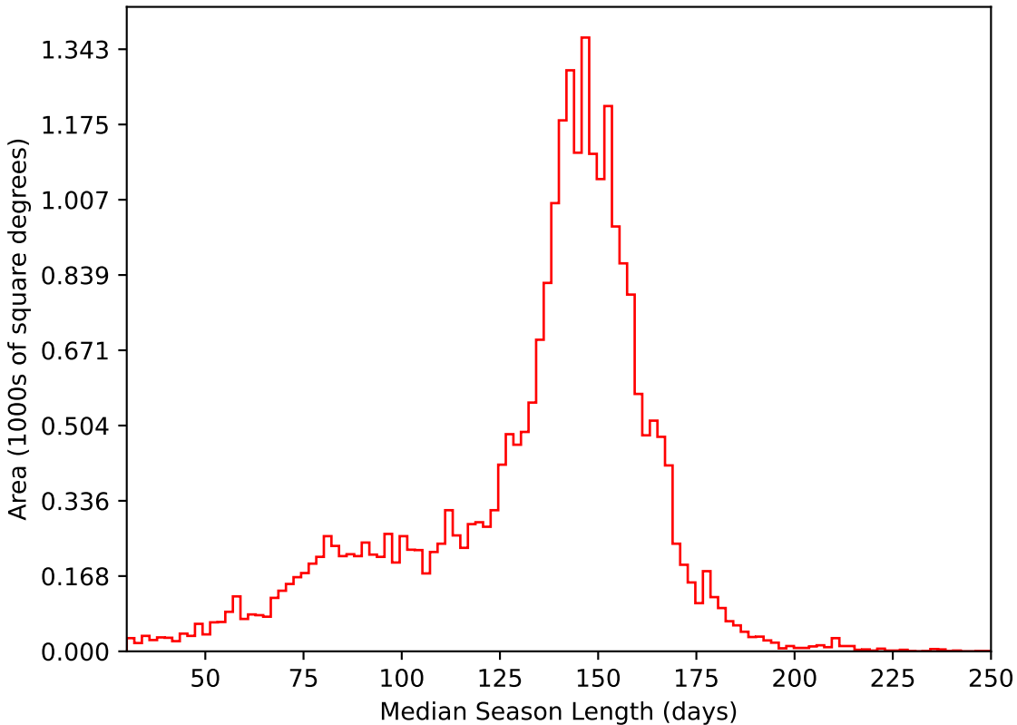
too_100_1v3.4_10yrs All sky i band: Median Season Length
