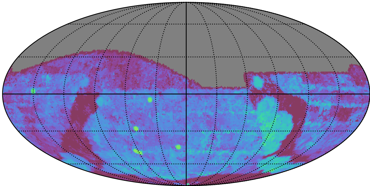
too_100_1v3.4_10yrs All sky g band: Median Season Length
