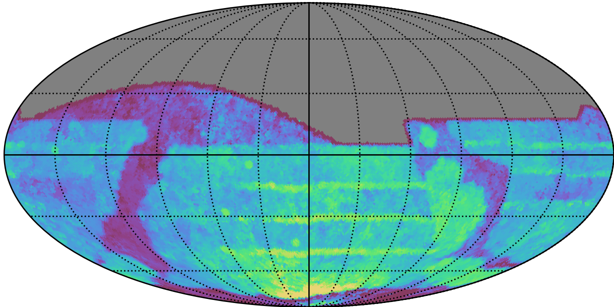
too_100_1v3.4_10yrs All sky all bands: Median Season Length
