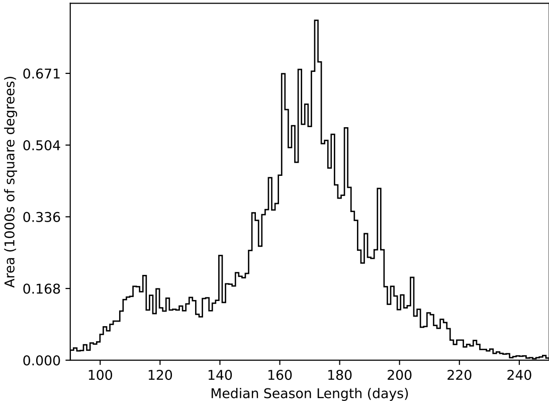
too_100_1v3.4_10yrs All sky all bands: Median Season Length
