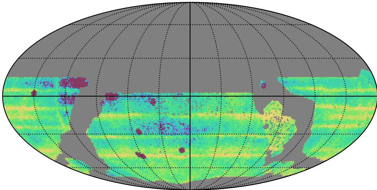
too_100_1v3.4_10yrs WFD: Median Intra-Night Gap
