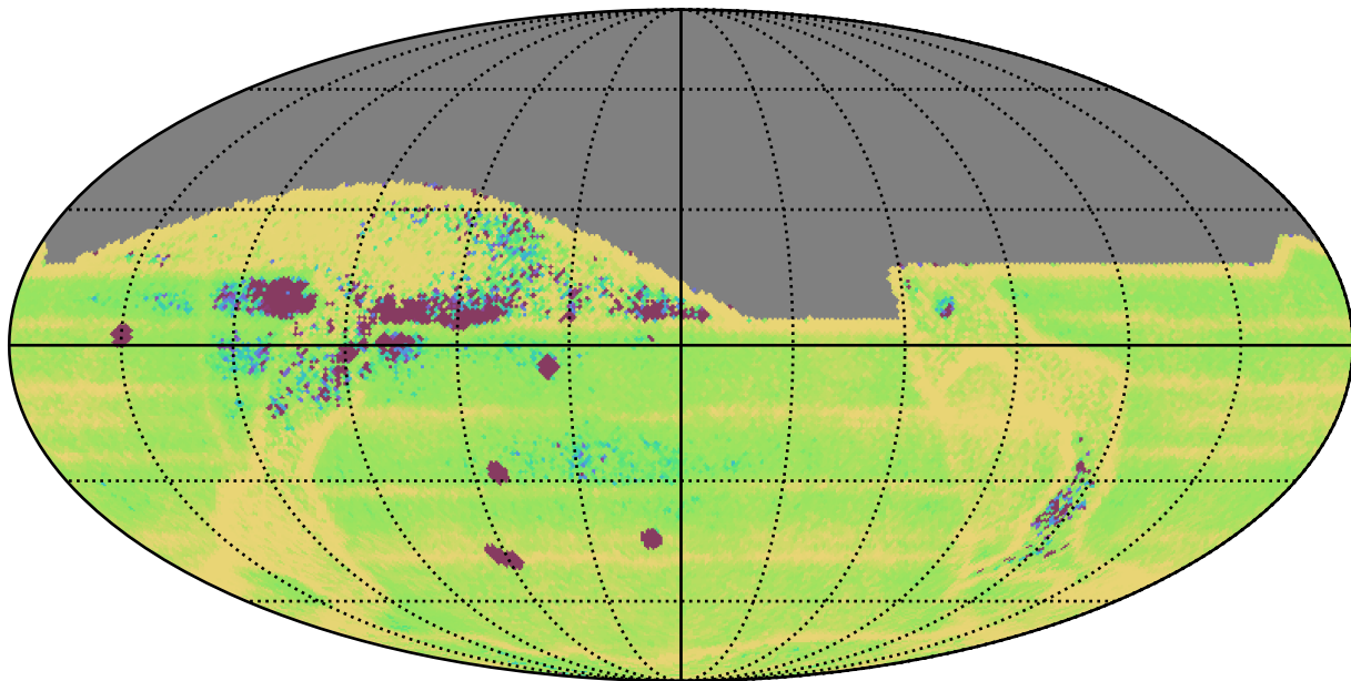
too_100_1v3.4_10yrs All sky: Median Intra-Night Gap
