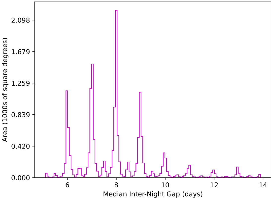
too_100_1v3.4_10yrs WFD z band: Median Inter-Night Gap
