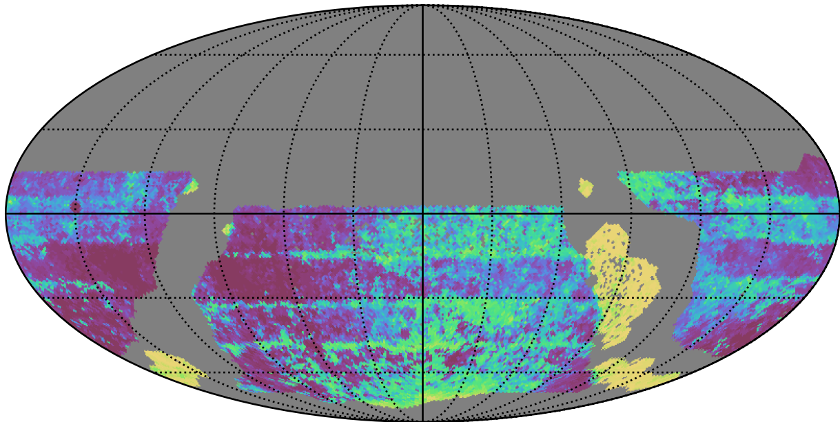
too_100_1v3.4_10yrs WFD y band: Median Inter-Night Gap
