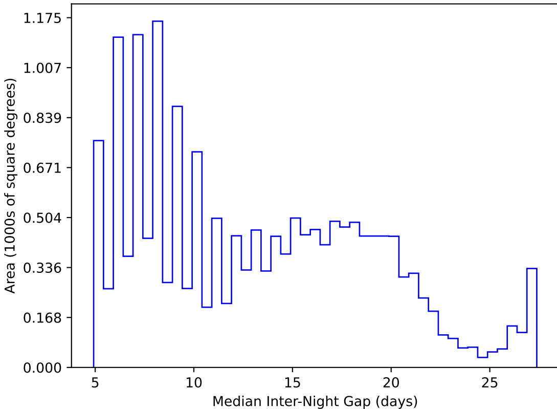
too_100_1v3.4_10yrs WFD y band: Median Inter-Night Gap
