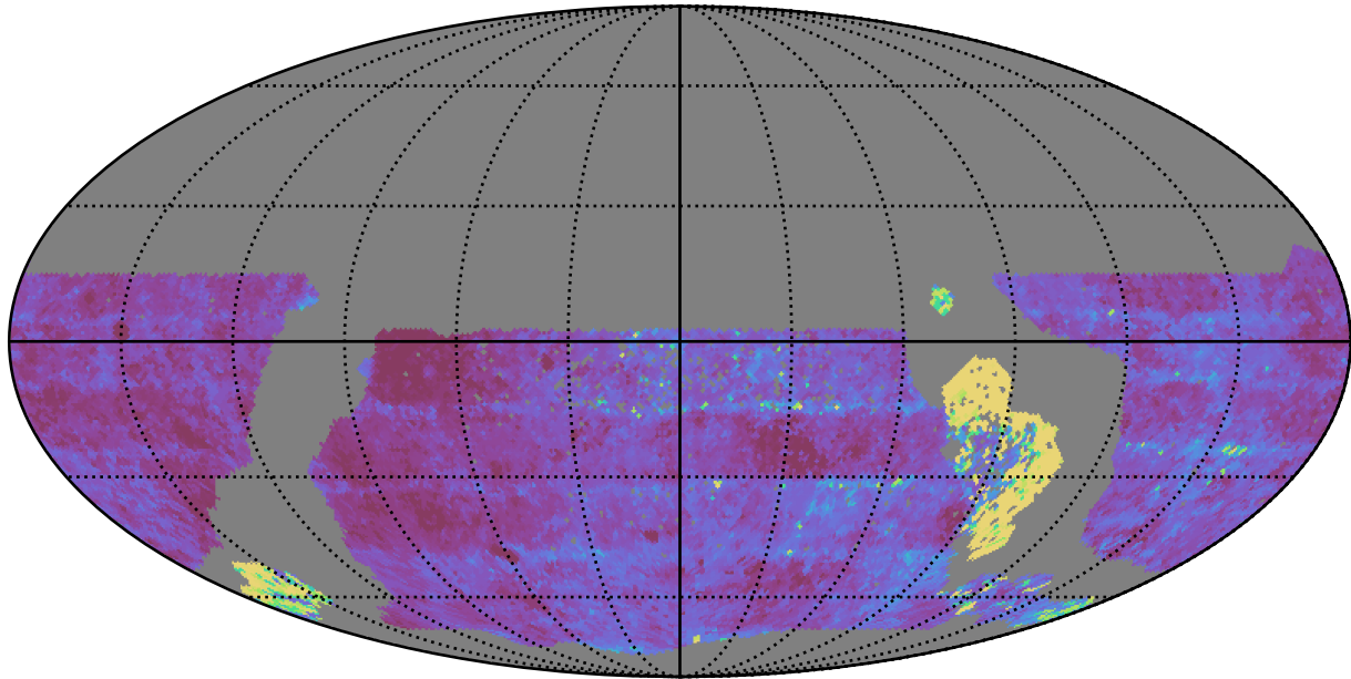
too_100_1v3.4_10yrs WFD u band: Median Inter-Night Gap
