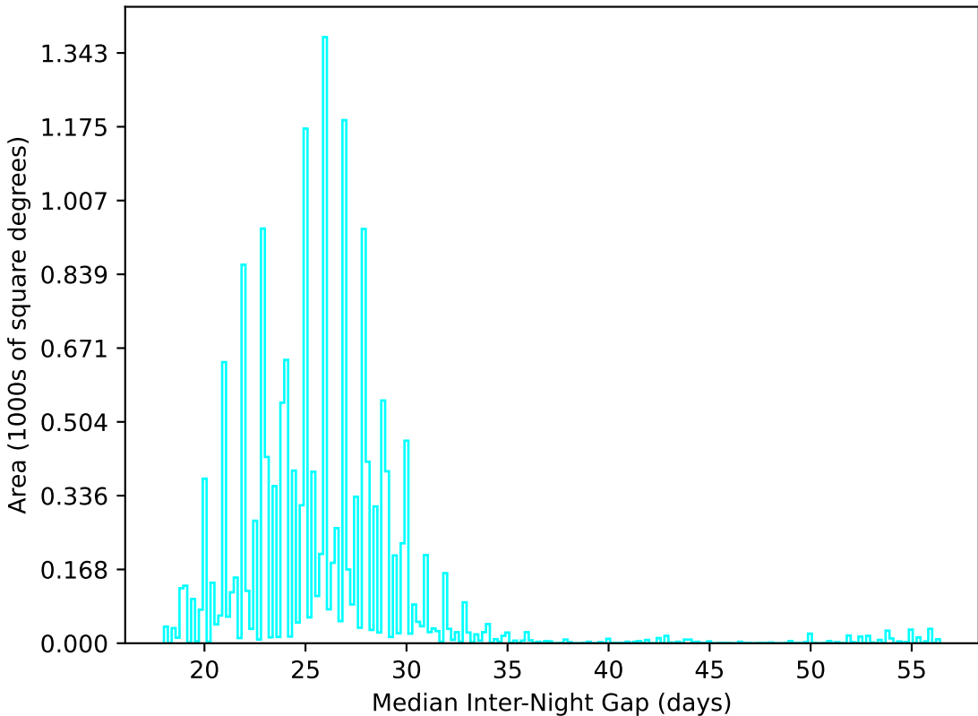
too_100_1v3.4_10yrs WFD u band: Median Inter-Night Gap
