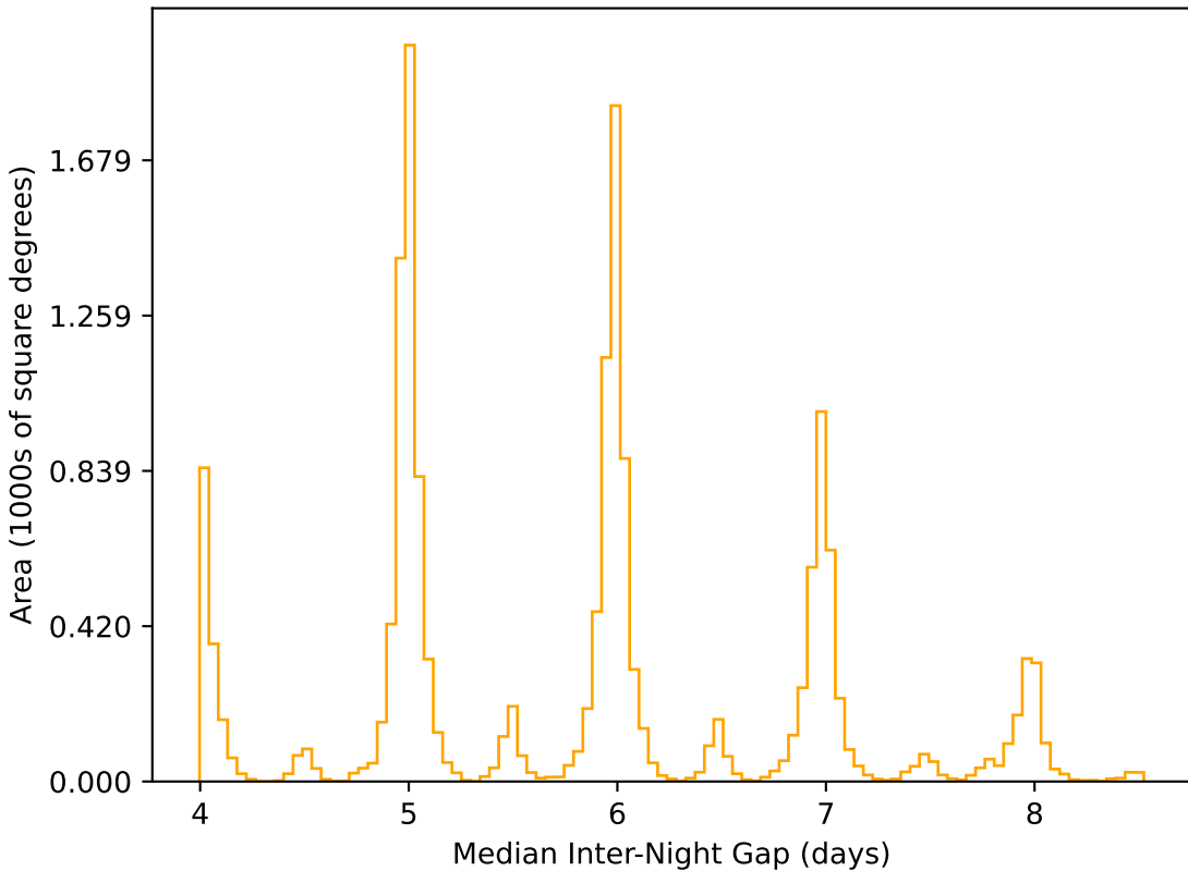
too_100_1v3.4_10yrs WFD r band: Median Inter-Night Gap
