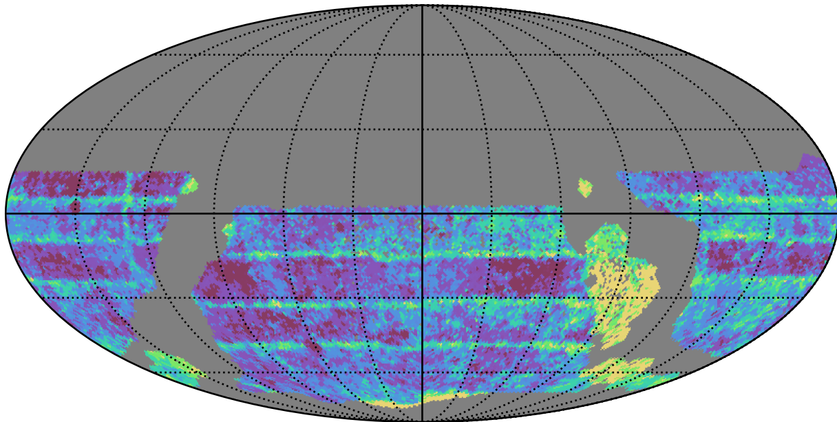
too_100_1v3.4_10yrs WFD i band: Median Inter-Night Gap
