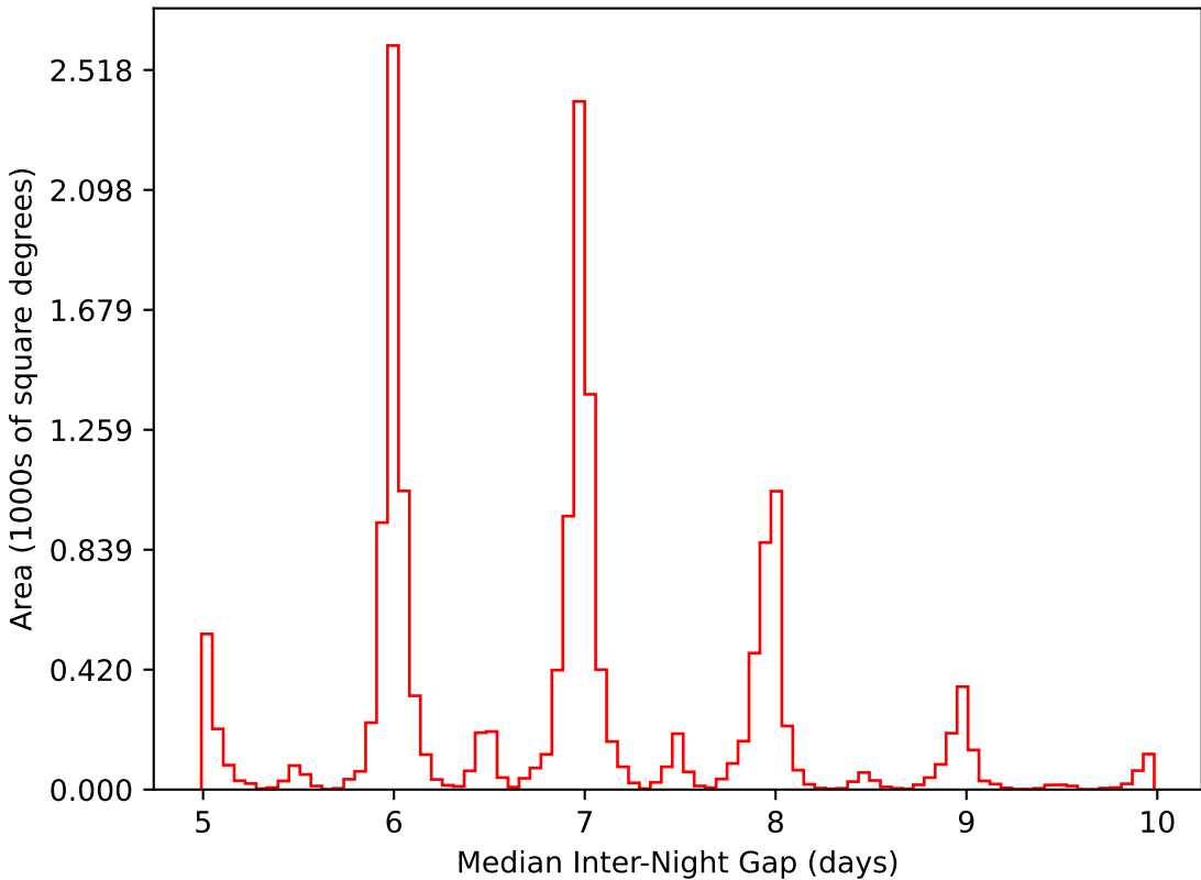
too_100_1v3.4_10yrs WFD i band: Median Inter-Night Gap
