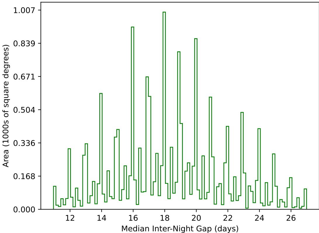
too_100_1v3.4_10yrs WFD g band: Median Inter-Night Gap
