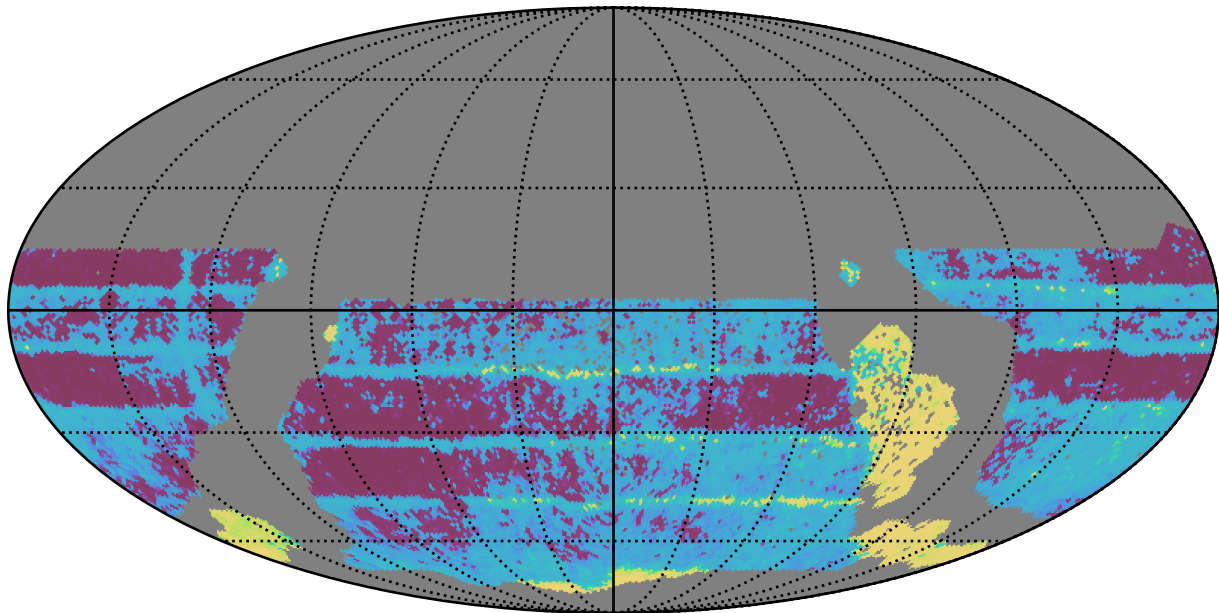
too_100_1v3.4_10yrs WFD all bands: Median Inter-Night Gap
