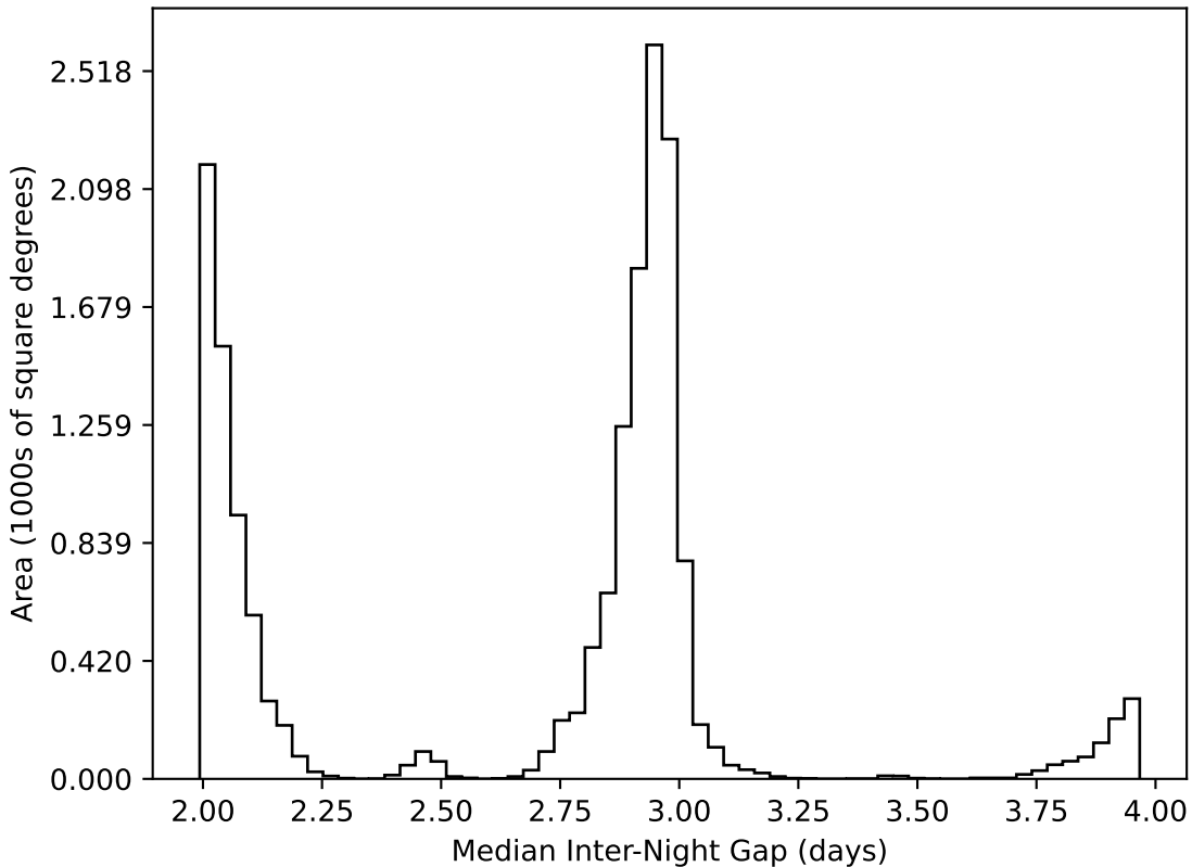
too_100_1v3.4_10yrs WFD all bands: Median Inter-Night Gap
