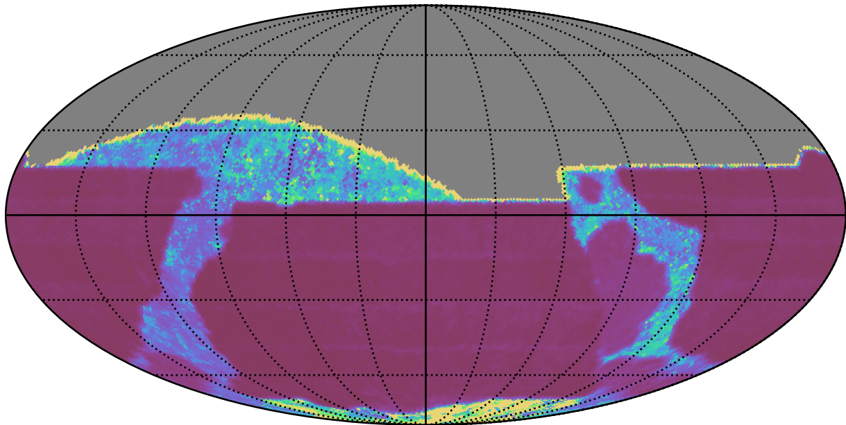
too_100_1v3.4_10yrs All sky z band: Median Inter-Night Gap
