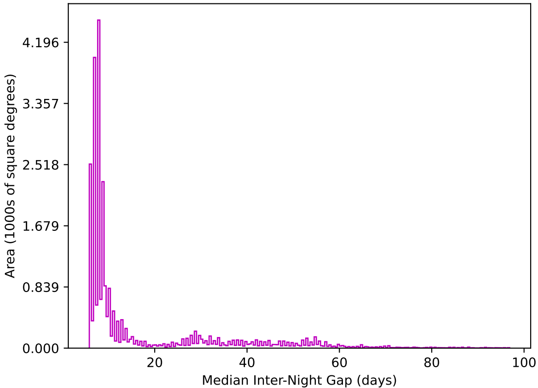
too_100_1v3.4_10yrs All sky z band: Median Inter-Night Gap
