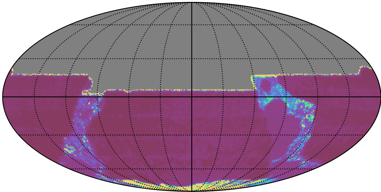
too_100_1v3.4_10yrs All sky y band: Median Inter-Night Gap
