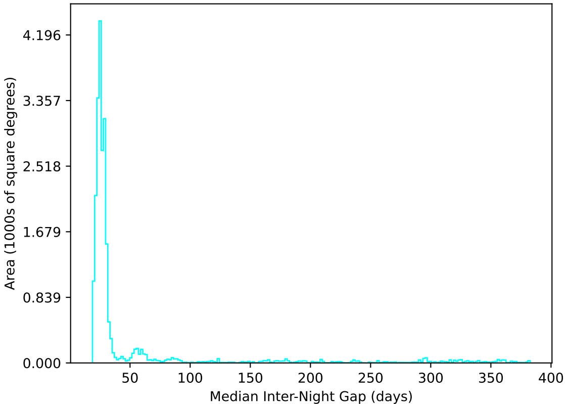
too_100_1v3.4_10yrs All sky u band: Median Inter-Night Gap
