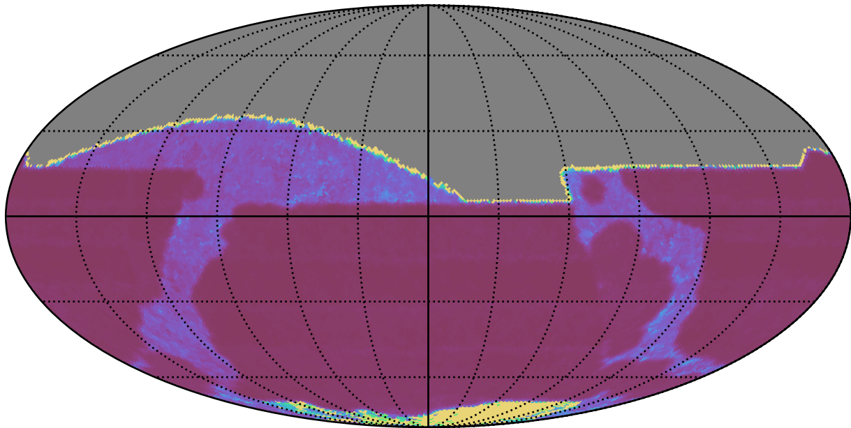
too_100_1v3.4_10yrs All sky r band: Median Inter-Night Gap
