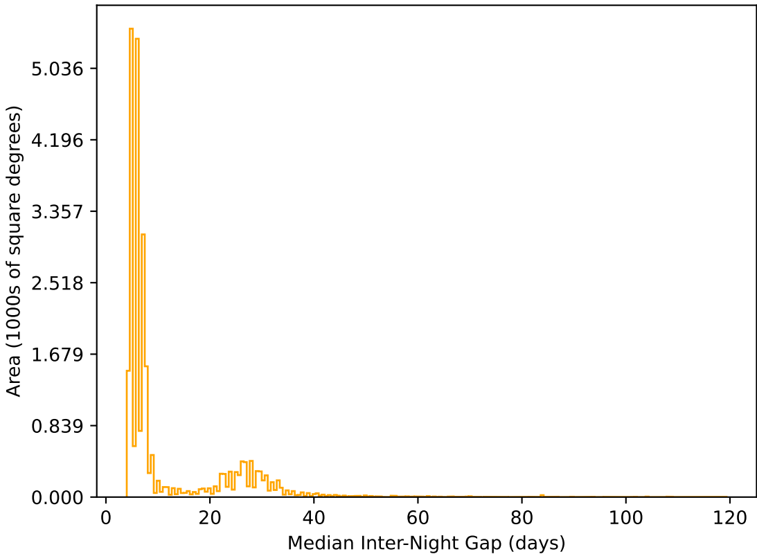
too_100_1v3.4_10yrs All sky r band: Median Inter-Night Gap
