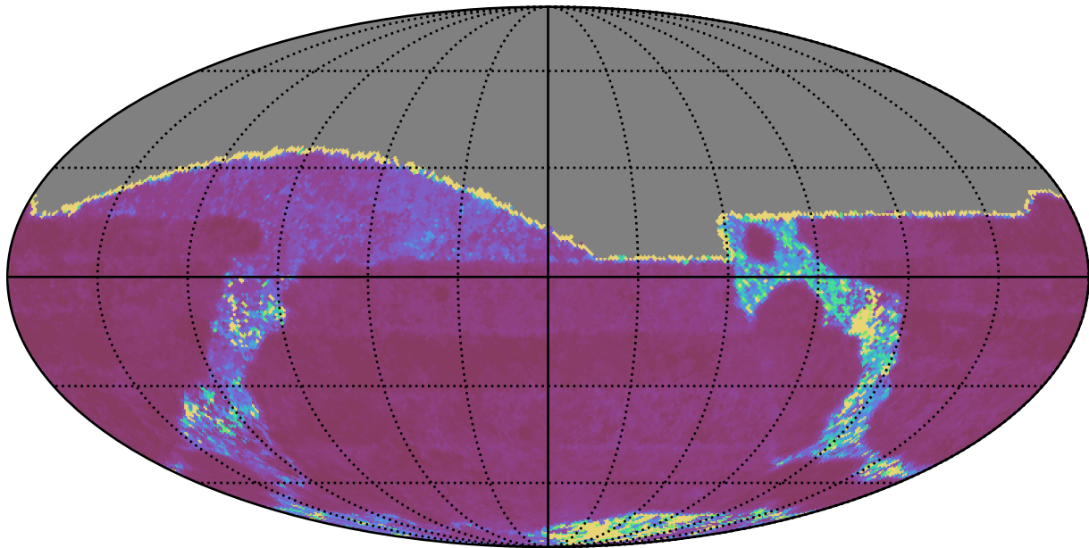
too_100_1v3.4_10yrs All sky g band: Median Inter-Night Gap
