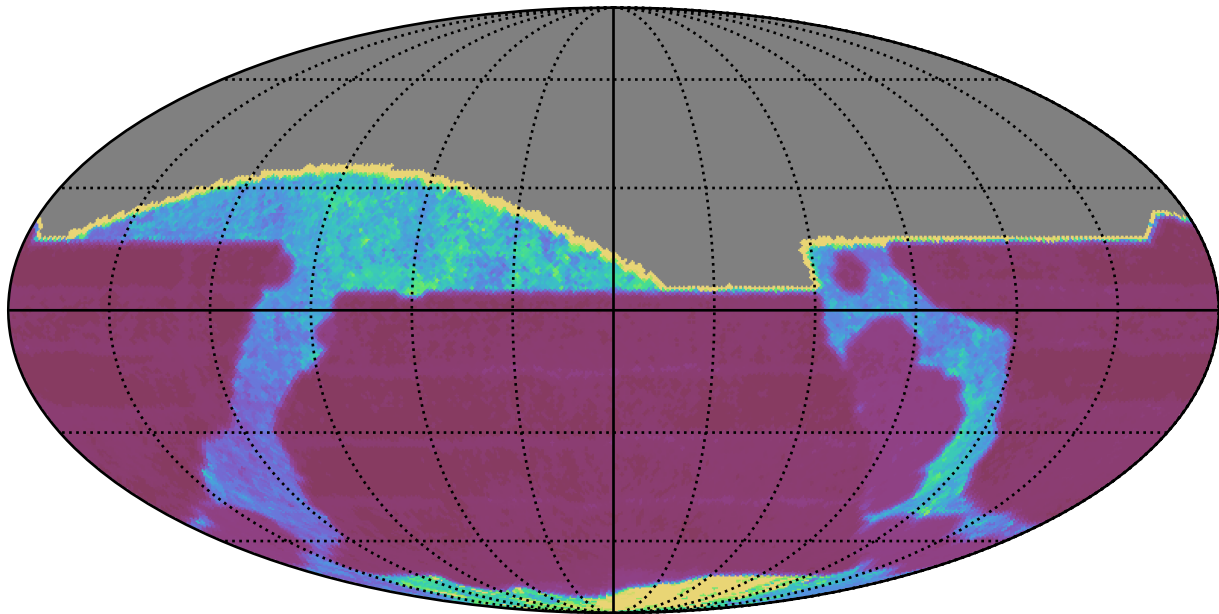
too_100_1v3.4_10yrs All sky all bands: Median Inter-Night Gap
