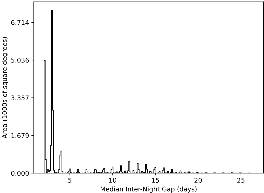
too_100_1v3.4_10yrs All sky all bands: Median Inter-Night Gap
