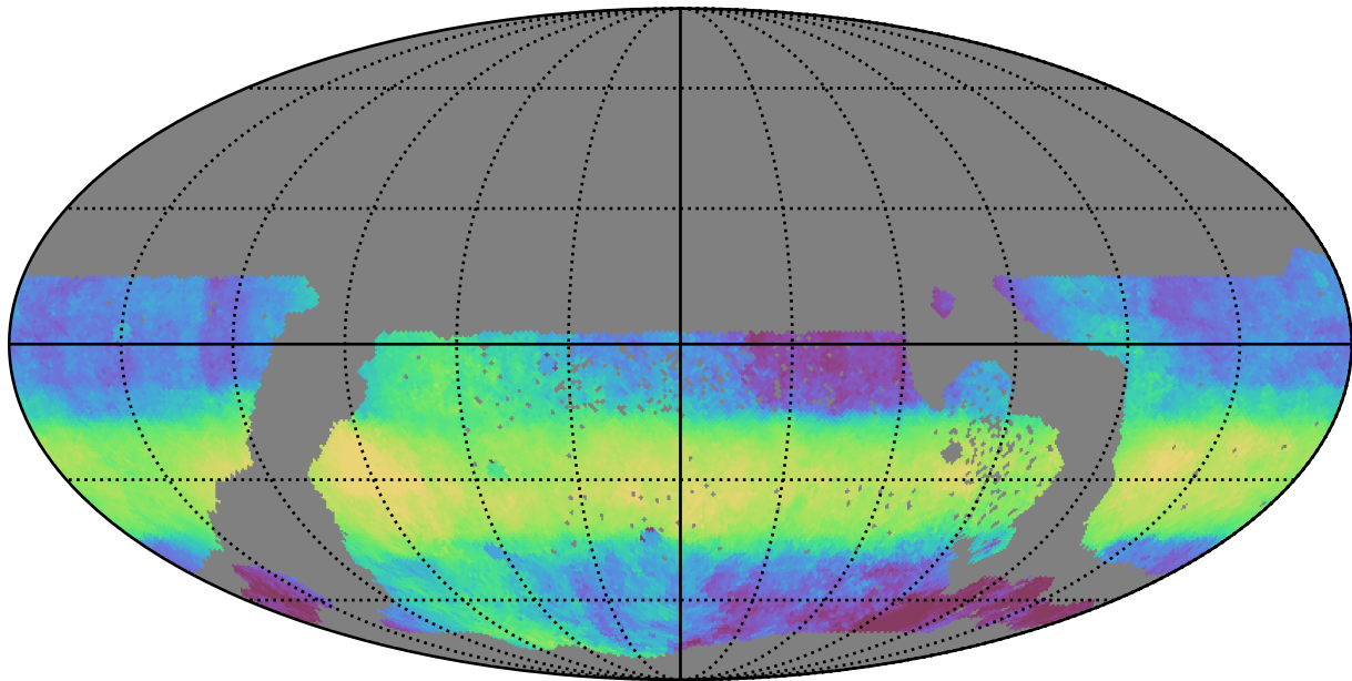
too_100_1v3.4_10yrs WFD z band: Median HA
