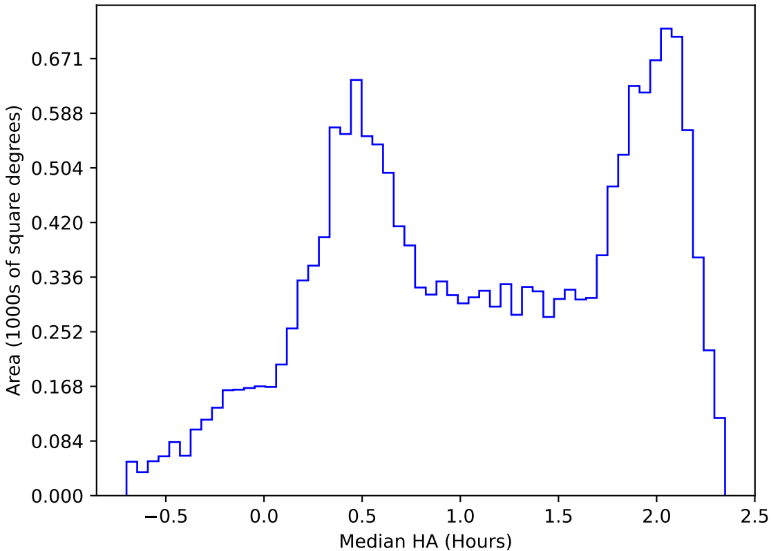
too_100_1v3.4_10yrs WFD z band: Median HA
