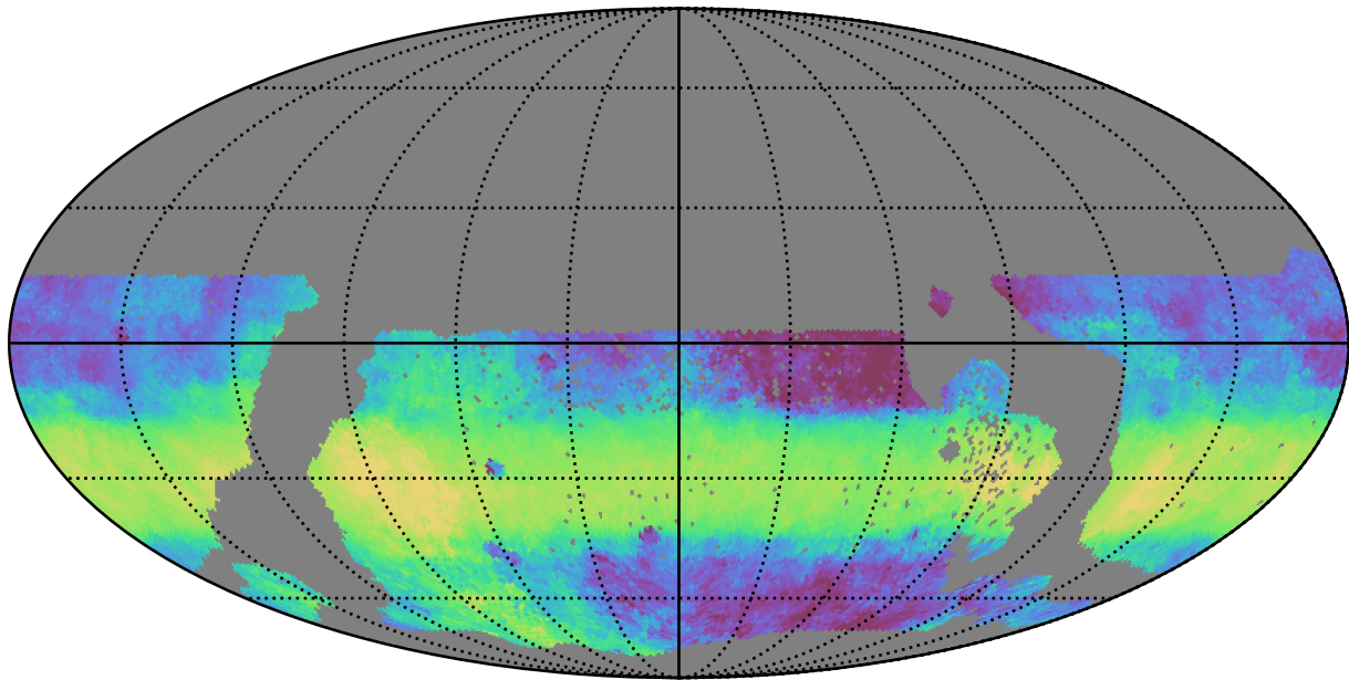
too_100_1v3.4_10yrs WFD y band: Median HA
