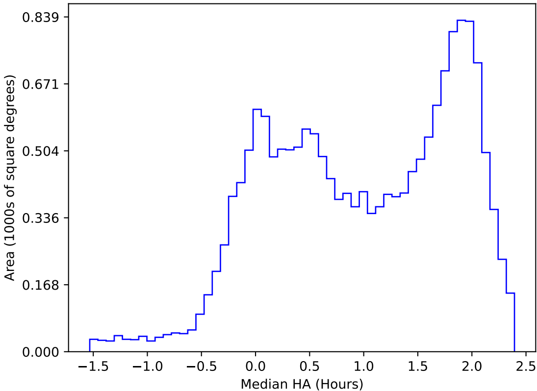
too_100_1v3.4_10yrs WFD u band: Median HA
