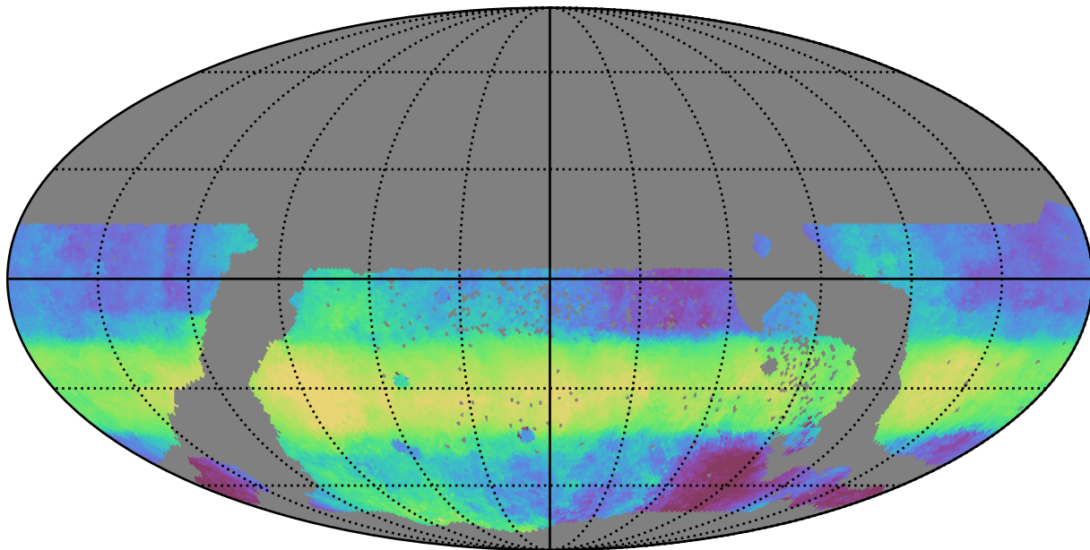
too_100_1v3.4_10yrs WFD r band: Median HA
