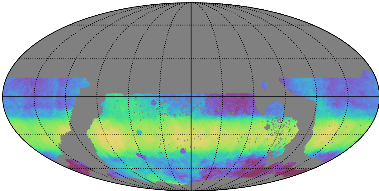
too_100_1v3.4_10yrs WFD i band: Median HA
