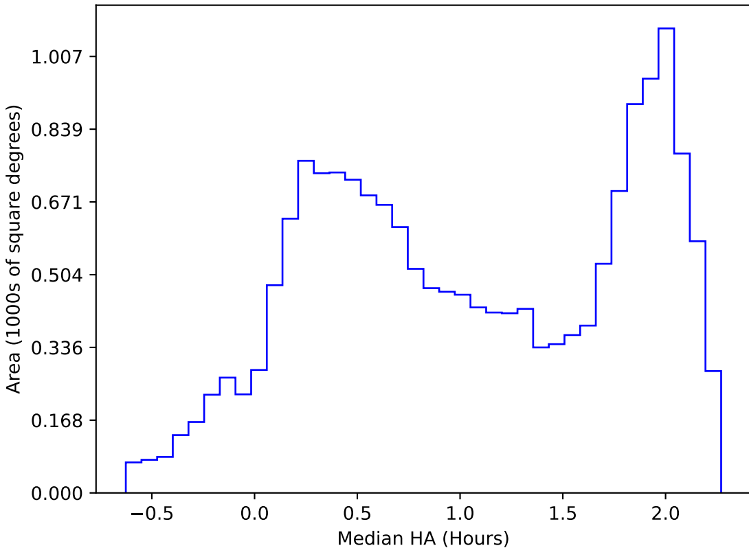
too_100_1v3.4_10yrs WFD i band: Median HA
