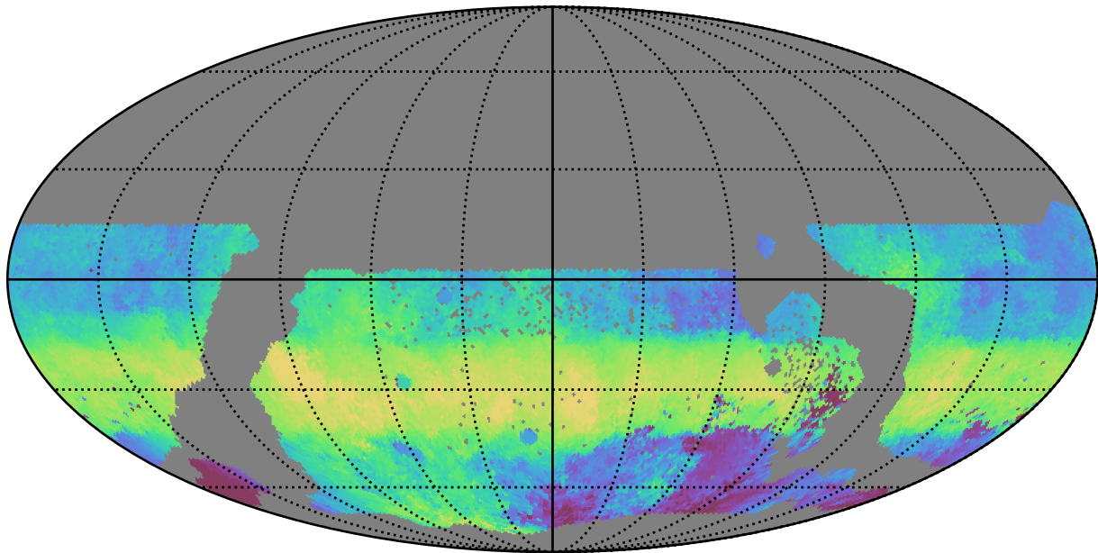
too_100_1v3.4_10yrs WFD g band: Median HA
