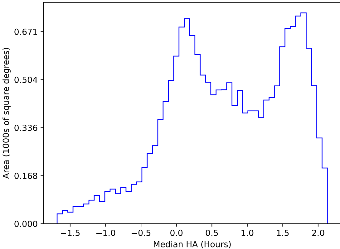
too_100_1v3.4_10yrs WFD g band: Median HA
