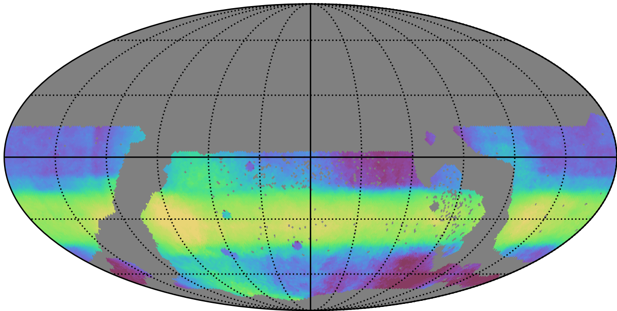
too_100_1v3.4_10yrs WFD all bands: Median HA
